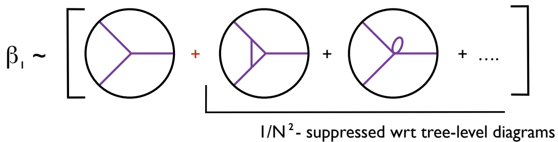
Figure 3.4. Witten diagrams contributing to C_{000} . Violet lines correspond to propagation of \phi fields and may have spacetime derivatives acting on them, depending on the specific structure of the operators (3.62). At tree-level, only cubic couplings can contribute to the three-point function. At loop level, also couplings with n > 3 can contribute, e.g. , the quintic coupling shown in the figure.
